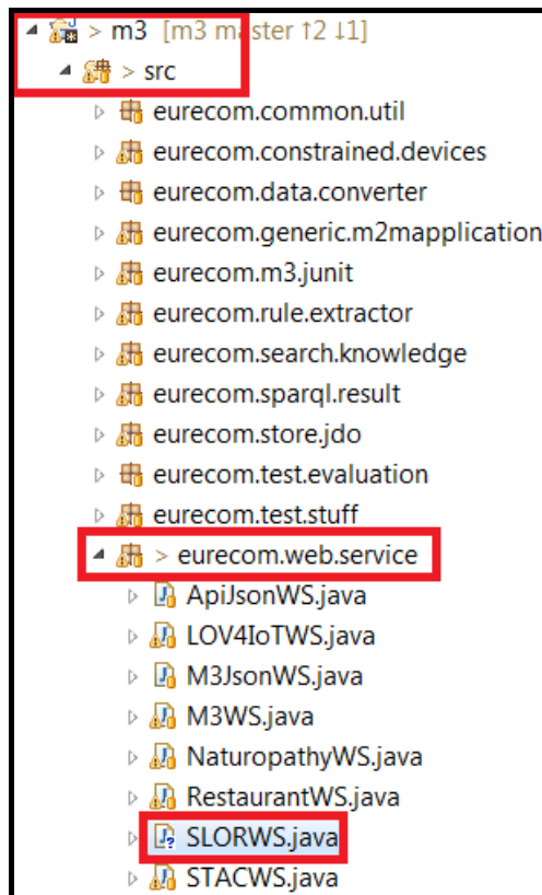
Figure 9. SLORWS.java file
